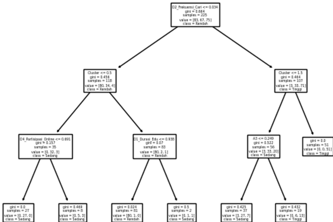
Gambar 7. Decision Tree
