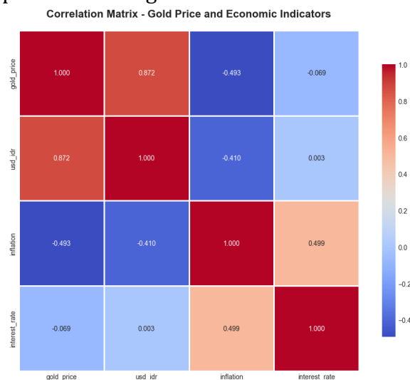
Gambar 7. Heatmap Correlation Matrix
