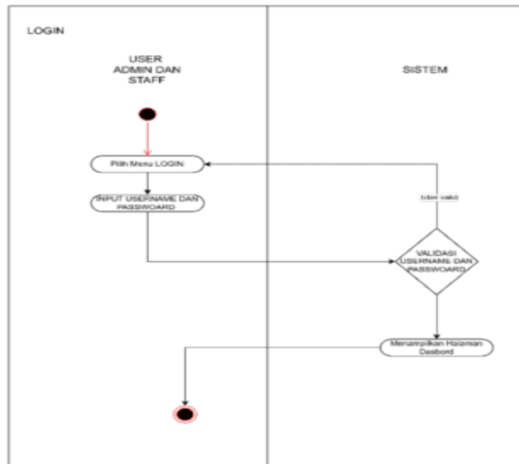
Gambar 4. Activity Diagram Login User
