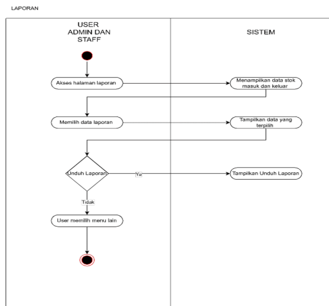
Gambar 7. Activity Diagram Menu Laporan Admin Dan Staff
