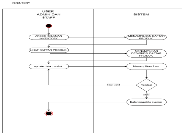
Gambar 6. Activity Diagram Menu Inventory Admin Dan Staff
