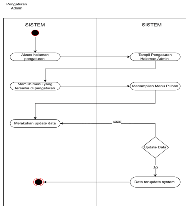
Gambar 8. Activity Diagram Menu Pengaturan Admin
