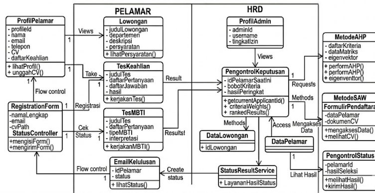
Gambar 5. Class diagram
