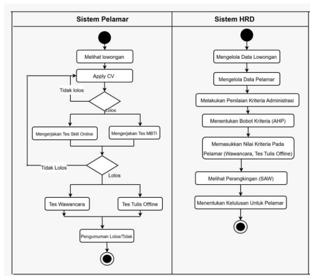
Gambar 4. Activity diagram
