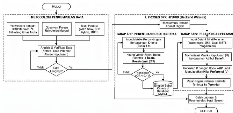
Gambar 2. Flowchart SPK metode hybrid
